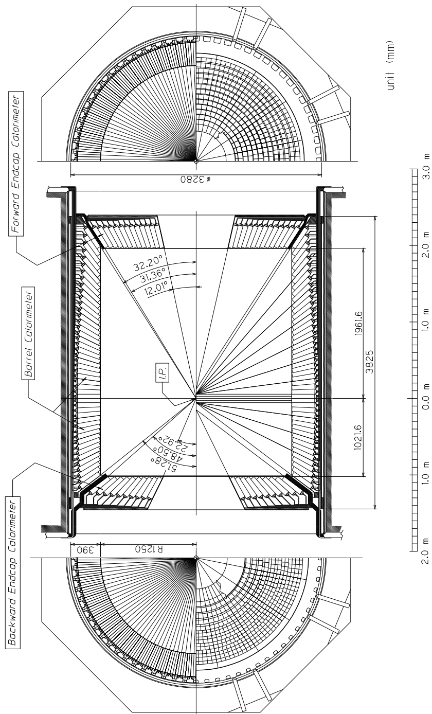
Figure 3.11: CsI calorimeter.
